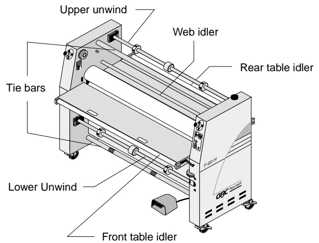
Figure 4.2.3 Idlers and unwinds
