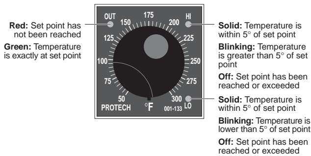
Figure 3-4: Heater Controller
