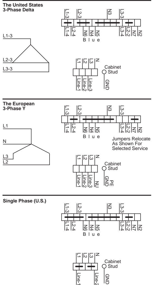
Figure 2-6: Power Cord Connection
