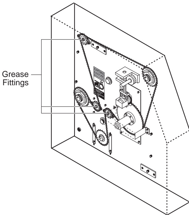
Figure 4-7: Grease Fittings
