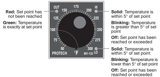
Figure 3-3: Heater Controller
