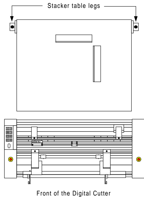
Figure 4.11.1 Positioning the stacker
