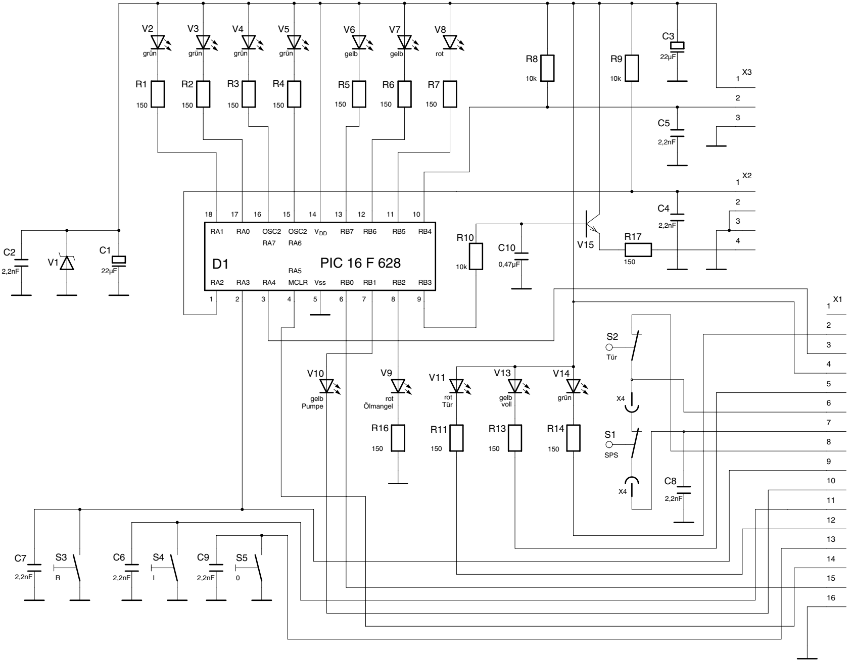
wiring diagram
