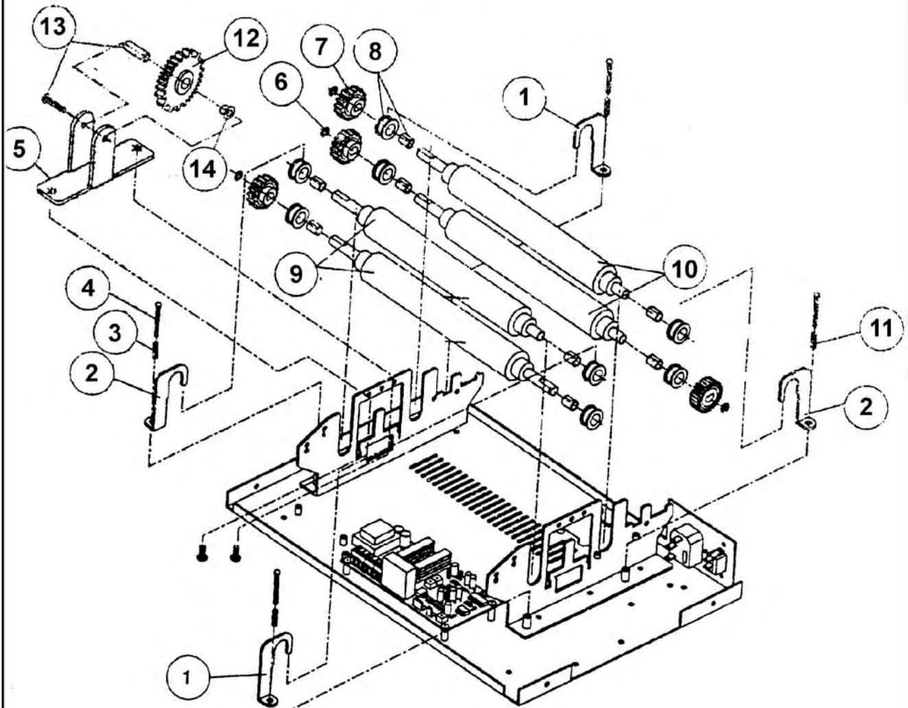
8.0 PARTS FIGURE 8.7
