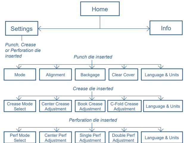
LCD Panel Overview
