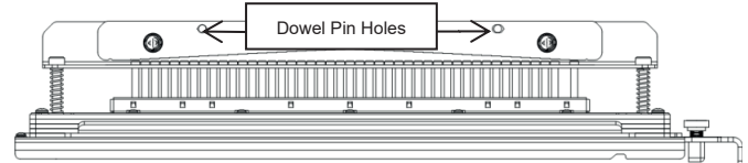
Figure 8.4 Replace Pressure Bar
