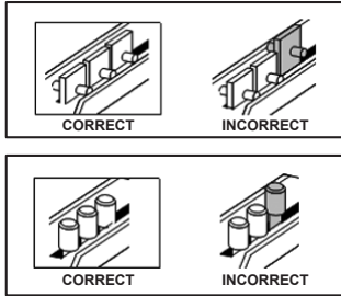
Figure 8.5 Pin Addition
