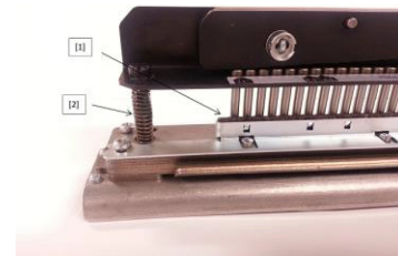
Figure 8.8 Lubrification
